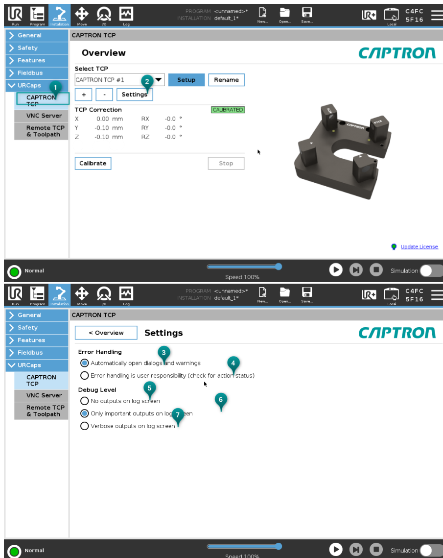
Abb. 25: URCap Settings
