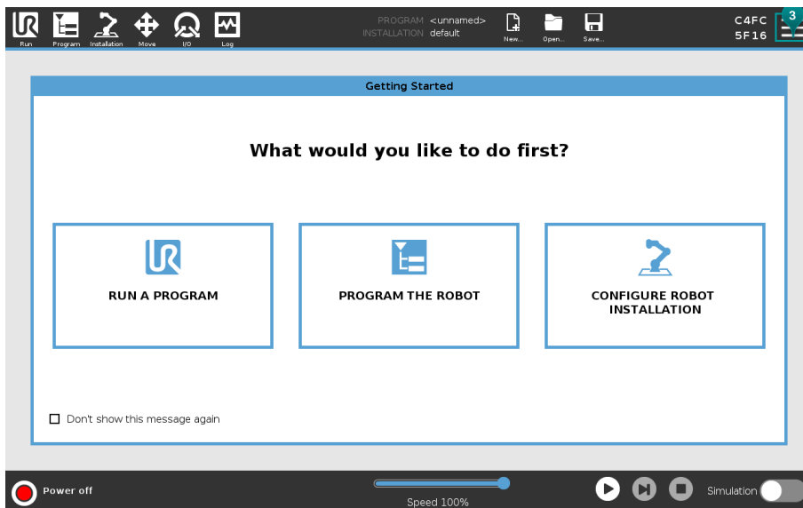
Abb. 1: Home screen
