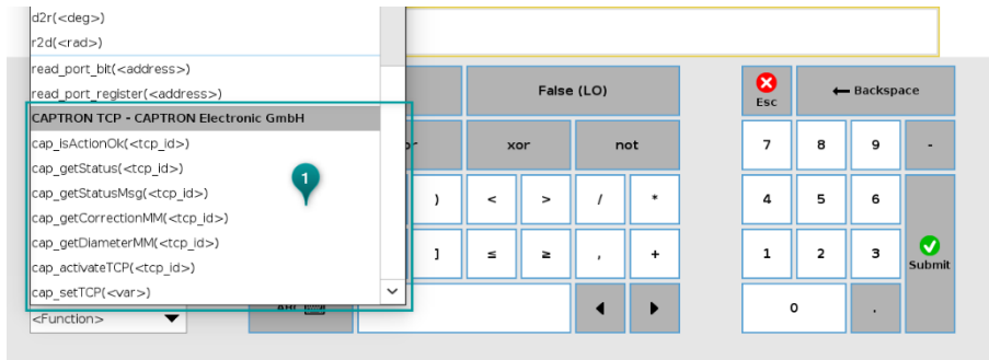
Abb. 36: Script Functions
