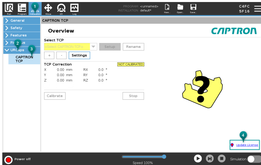
Abb. 8: Installation page
