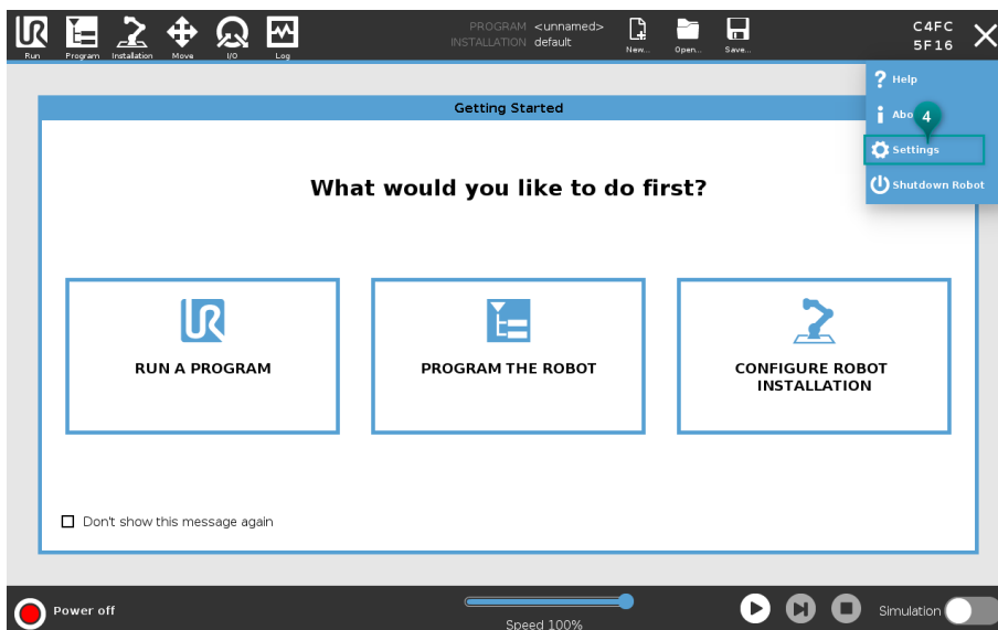
Abb. 2: Select Settings
